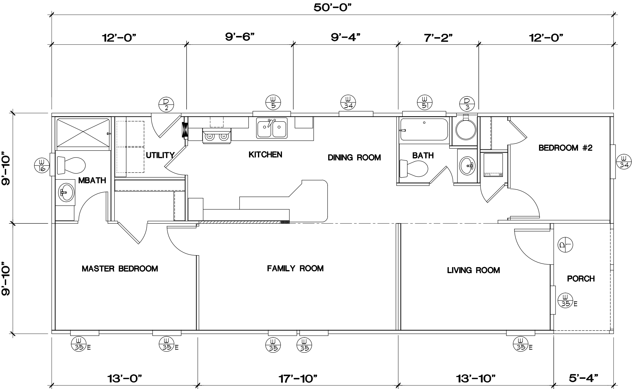
GP482P SPECIAL - 37630 930 SQ. FT.
